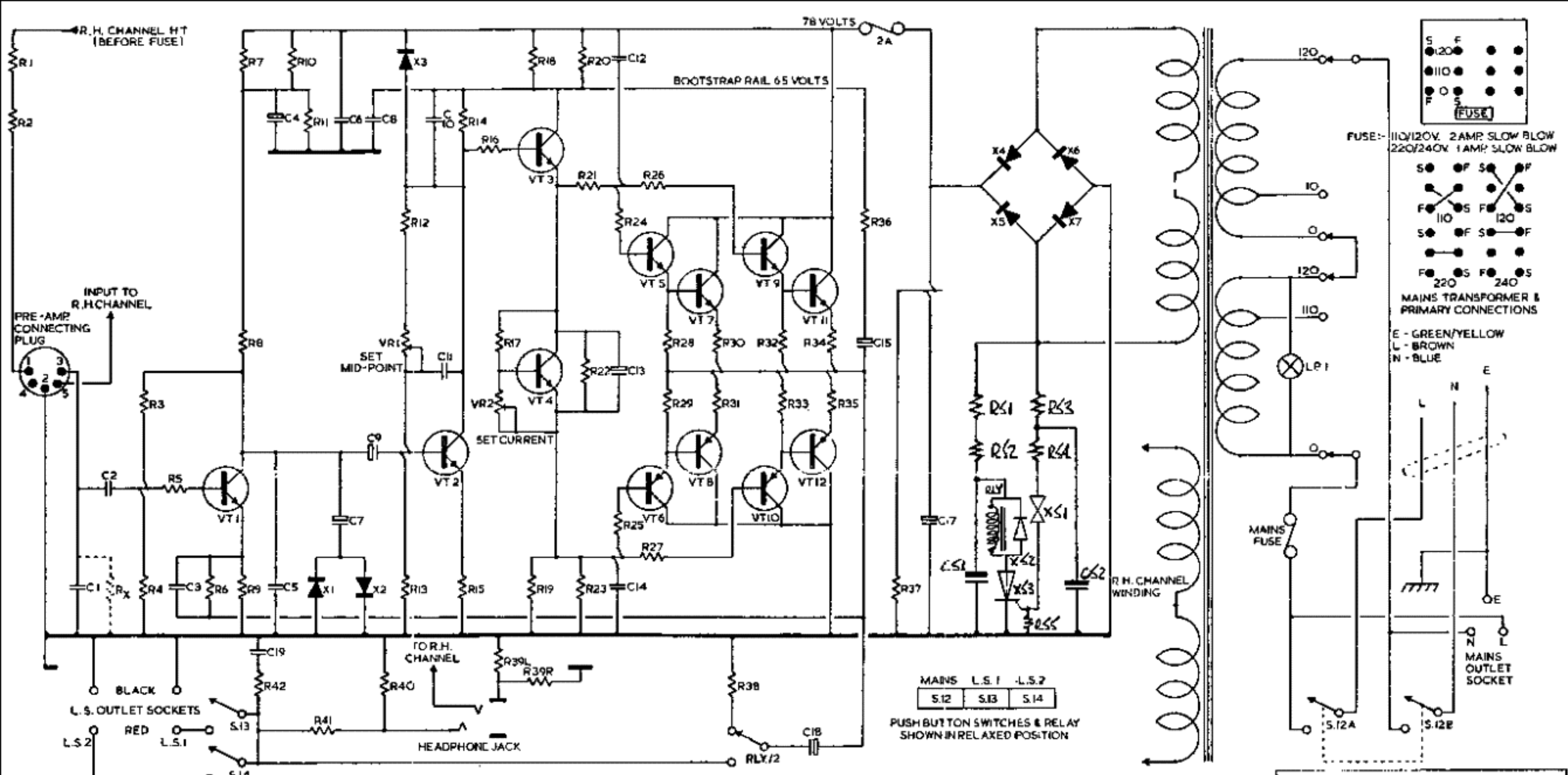
— POWER AMPLIFIER -A48— (L.H. CHANNEL SHOWN IN DETAIL)
